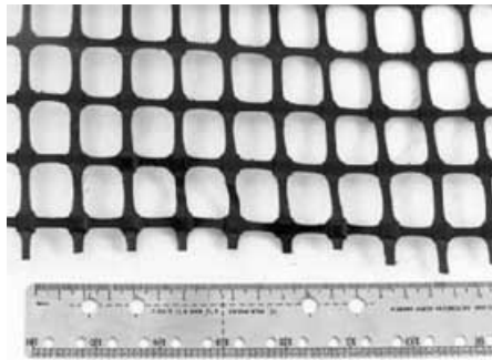
Figure 4. Geogrid for heavy traffic areas.
