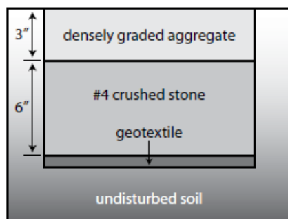
Figure 1. Construction details.
